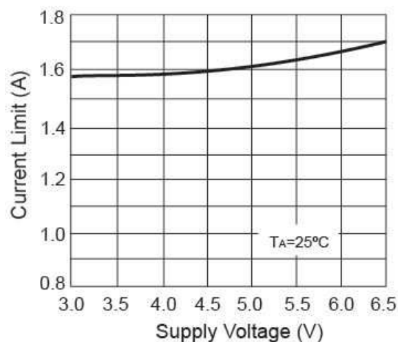
Figure 5. Current Limit vs. Supply Voltage
