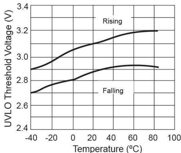
Figure 10. UVLO Threshold vs. Temperature
