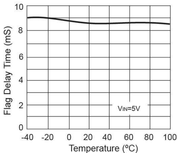
Figure 8. Flag Delay Time vs. Temperature
